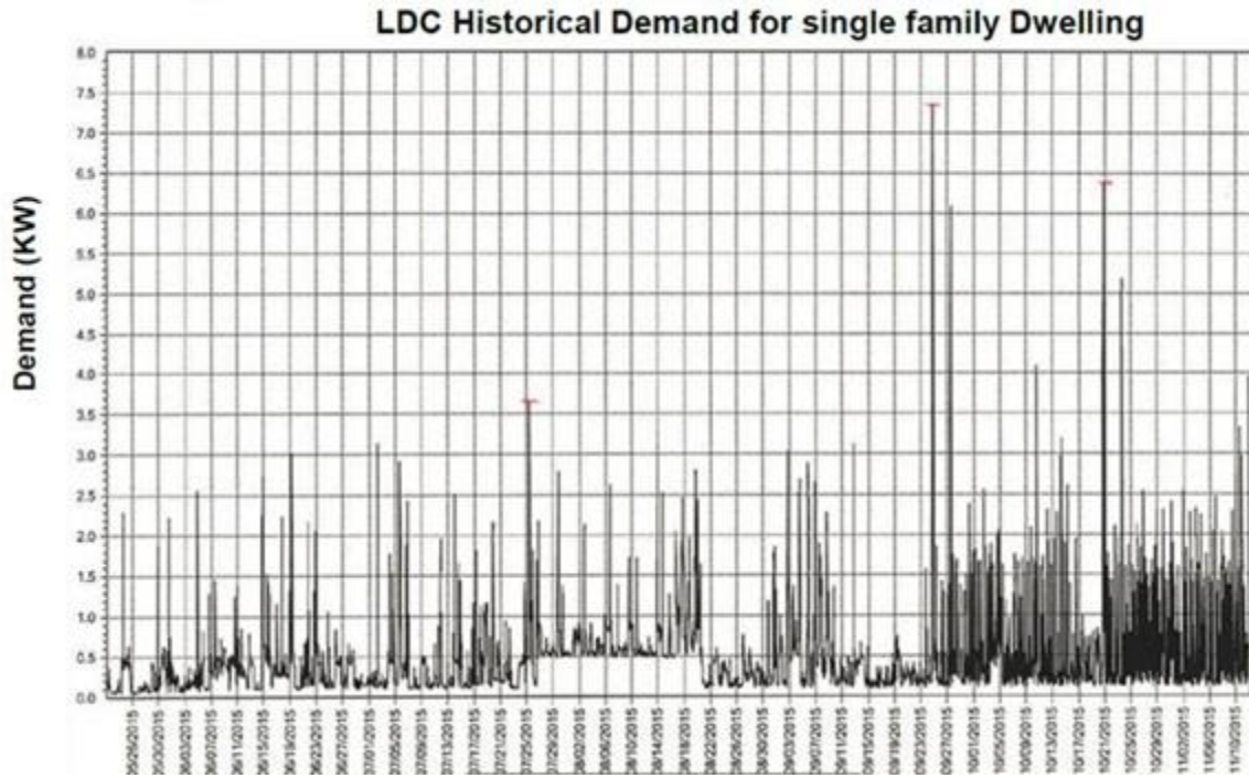
Diagram B1 – Example, LDC Historical Demand over the last 12 months for single-family dwelling
